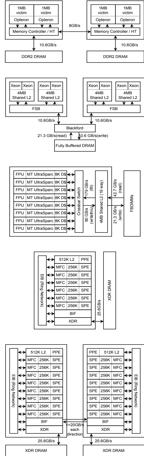
Figure 2: Architectural overview of (a) dual-socket x dual-core AMD Opteron X2 (b) dual-socket x quad-core Intel Clovertown, (c) single-socket x eight-core Sun Niagara2 (d) single-socket x six-core STI PS3 and (e) dual-socket x eight-core STI Cell.
